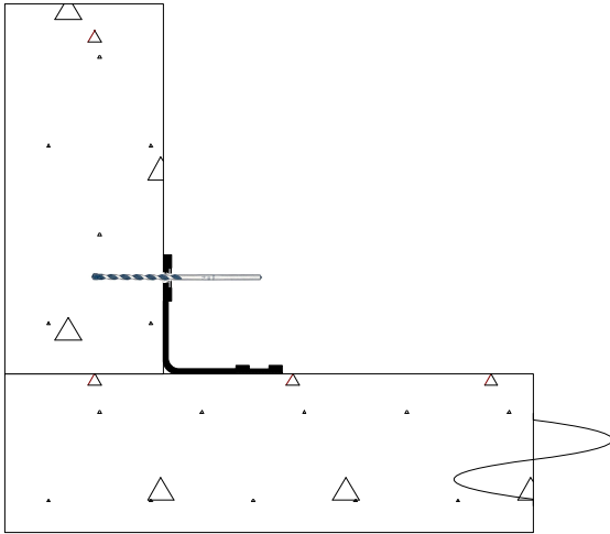
5) Using the prepunched stainless steel batten bar as a template, drill 1/4" holes 2-3/4" deep through waterstop and concrete. Clean out holes.
