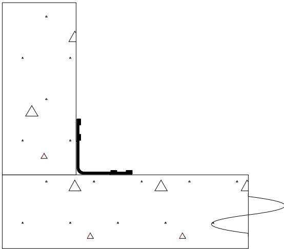
8) Embed waterstop into strips of uncured epoxy.
