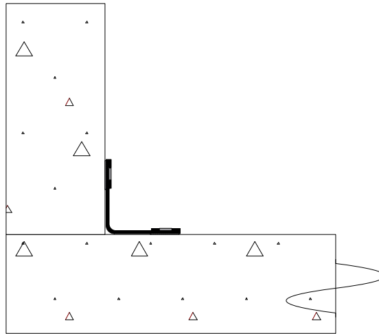
9) Place stainless steel batten bar in recesses of retrofit waterstop top and bottom.
