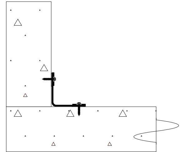
10) Install fasteners through predrilled holes in batten bar and waterstop and tighten as required.
